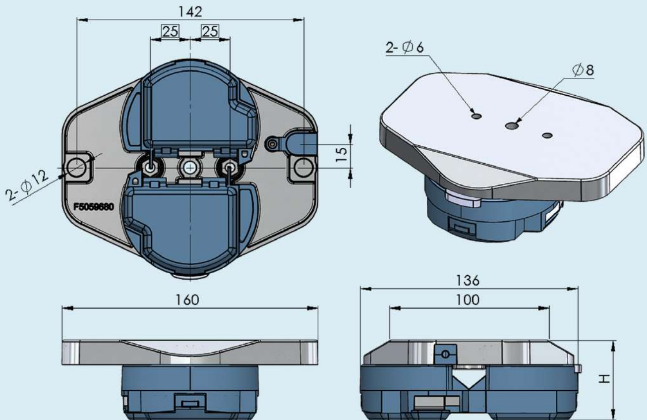
Pallet 160 x 100
