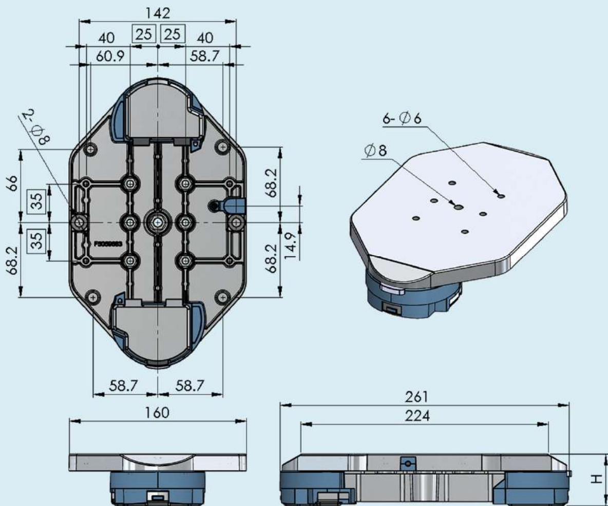
Pallet 160 x 225
