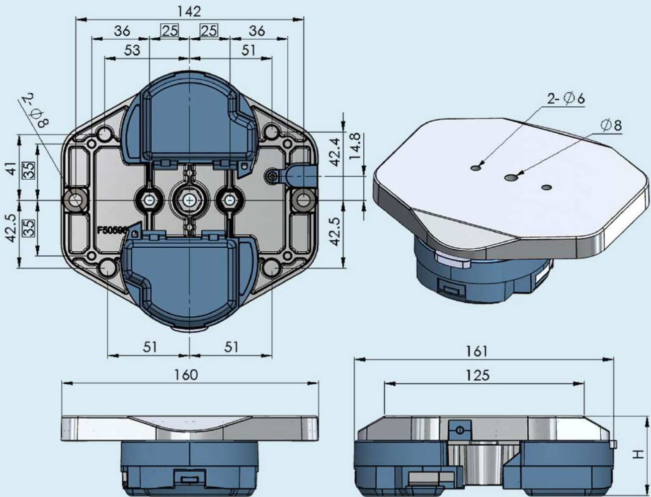
Pallet 160 x 125
